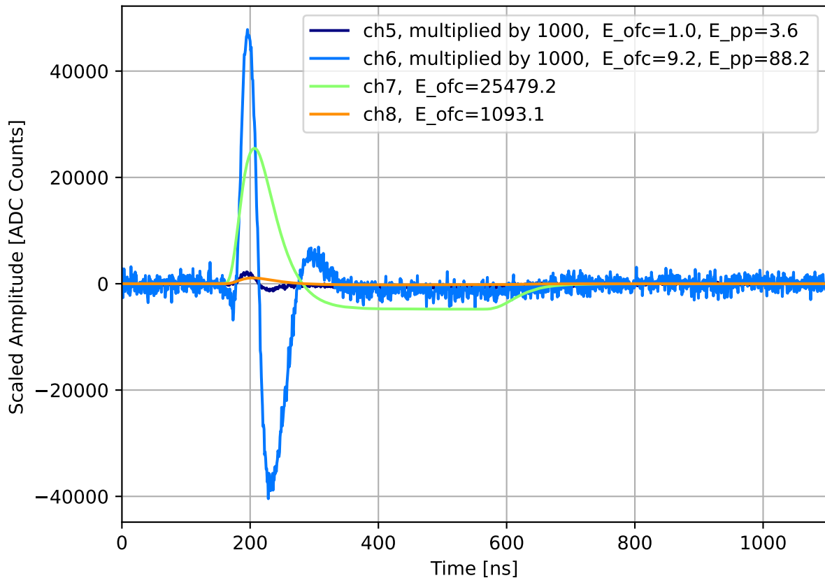
Run 2105, channel7, Crosstalk Pulses w/ 20.0 dB Attenuation
