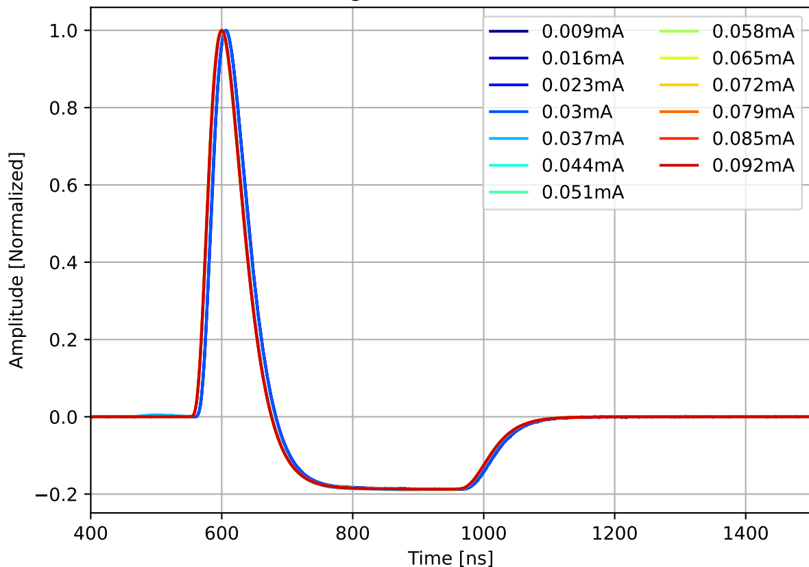
Run 2106, channel7, hi gain, Norm. Pulses w/ 27.0 dB Attenuation
