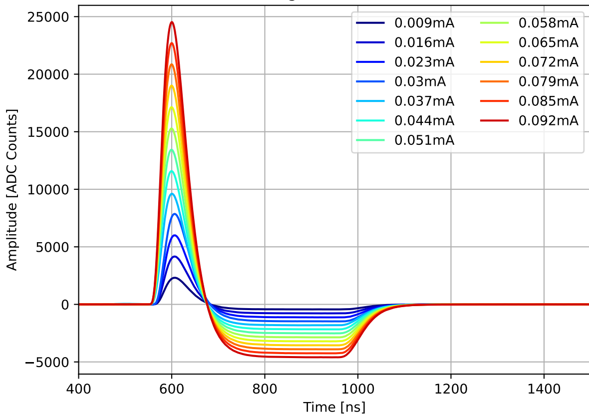
Run 2106, channel7, hi gain, Pulses w/ 27.0 dB Attenuation
