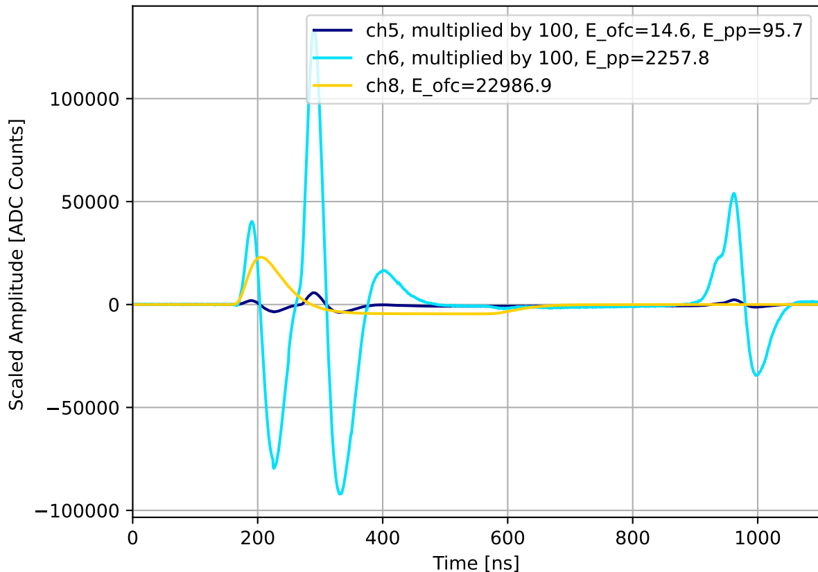
Run 2101, channel8, Crosstalk Pulses w/ 0.0 dB Attenuation
