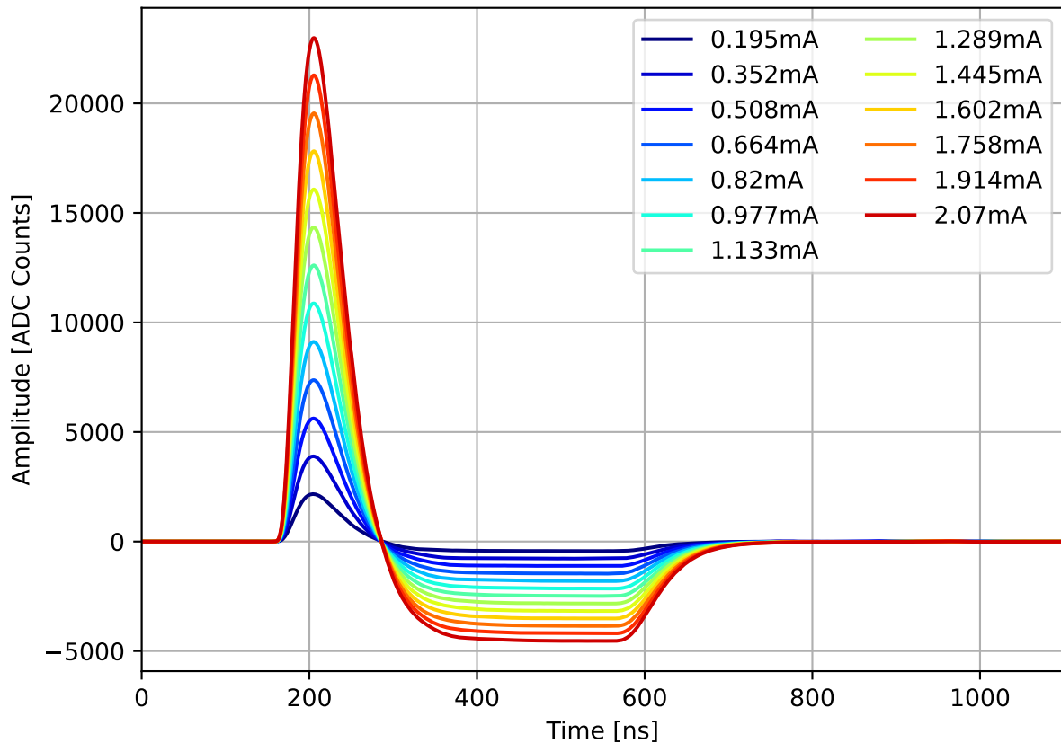
Run 2101, channel8, lo gain, Pulses w/ 0.0 dB Attenuation
