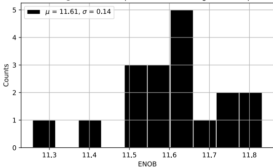
ENOB @ FS, Sine Freq.: 5.005 MHz, Configurable Chips
