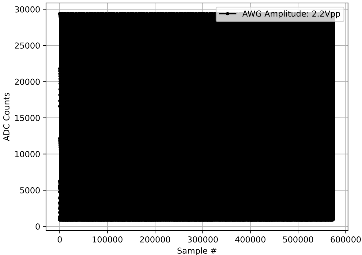
Run 2675, channel5, lo, Pulse w/ 6.0 dB Attenuation
