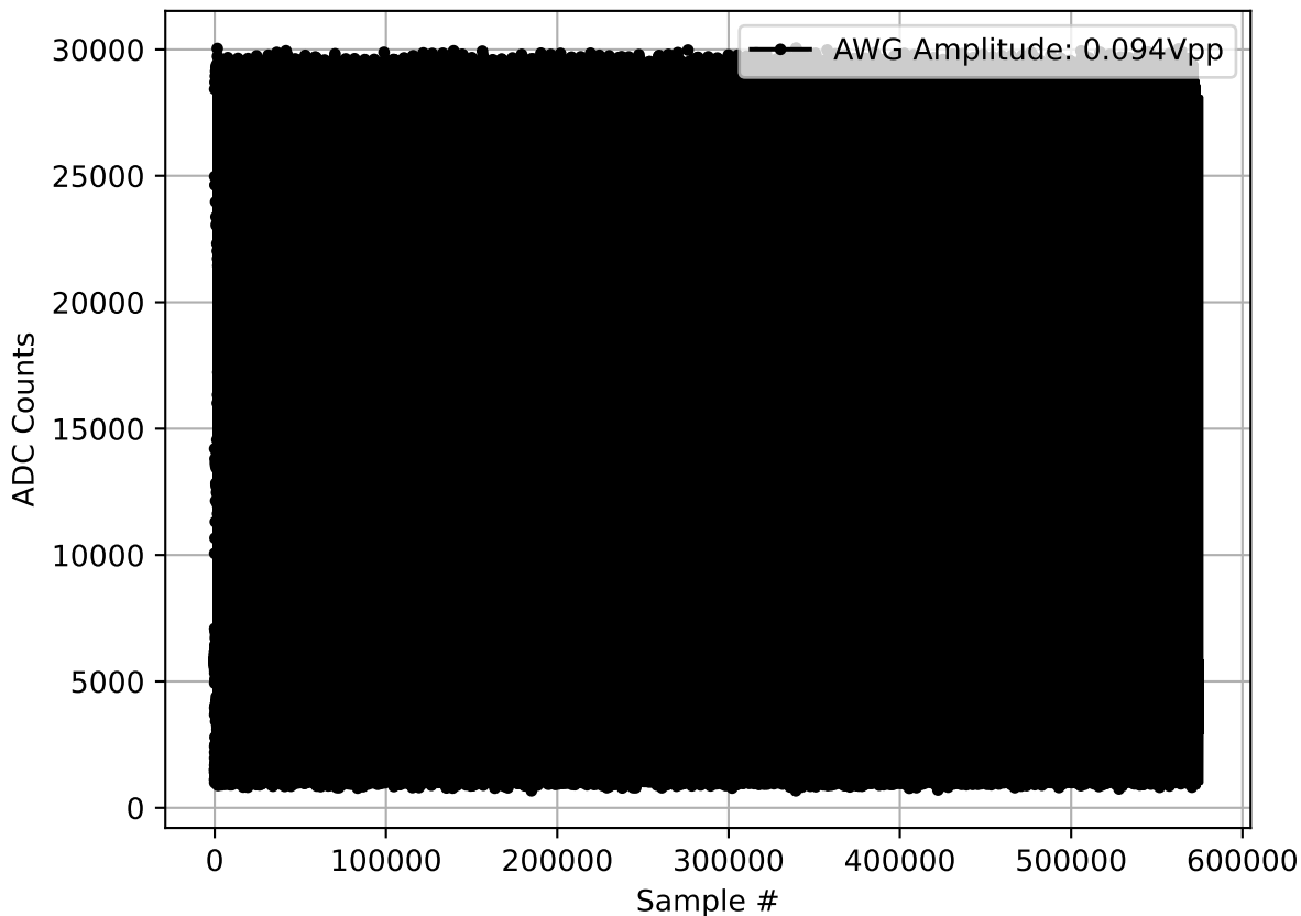
Run 2695, channel6, hi, Pulse w/ 6.0 dB Attenuation
