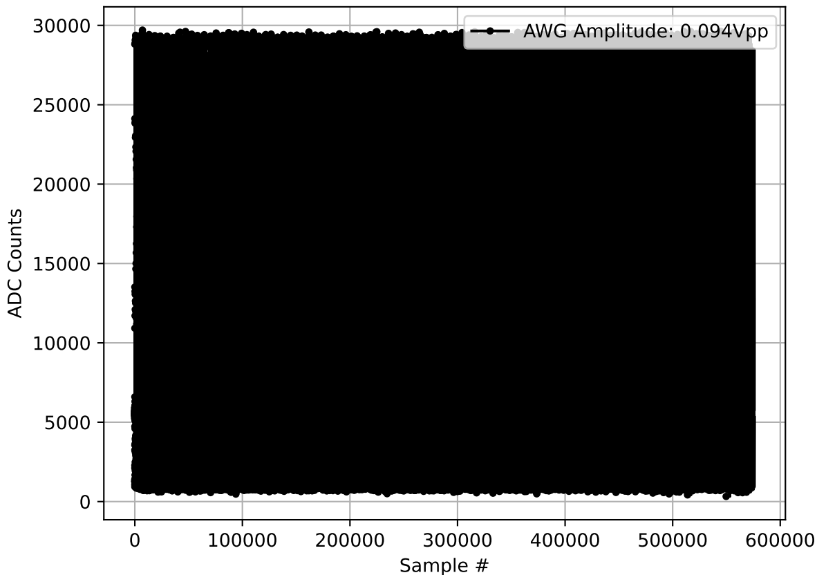
Run 2702, channel6, hi, Pulse w/ 6.0 dB Attenuation
