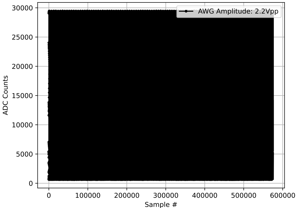
Run 2702, channel5, lo, Pulse w/ 6.0 dB Attenuation
