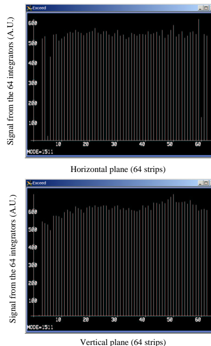
Fig. 3. Gain uniformity of the triple GEM monitor with a 70/30 ArCO 2 gas mixture irradiated by ^{90}\text{Sr} .
