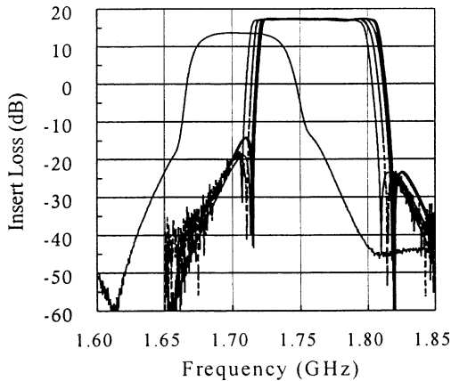
Fig. 1. Frequency responses of the HTS filters at different temperatures (from left to right: 86, 80, 77, 75, 71, 69 and 66 K).
