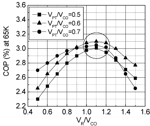
Fig. 2. COP as a function of regenerator volume and pulse tube volume of PTC.
