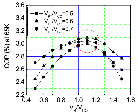
Figure 2 COP as a function of regenerator volume and pulse tube volume of PTC
