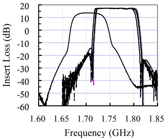
Figure 1 Frequency responses of HTS filters (from left to right: 86K, 80K, 75K, 71K, 69K and 66K)
