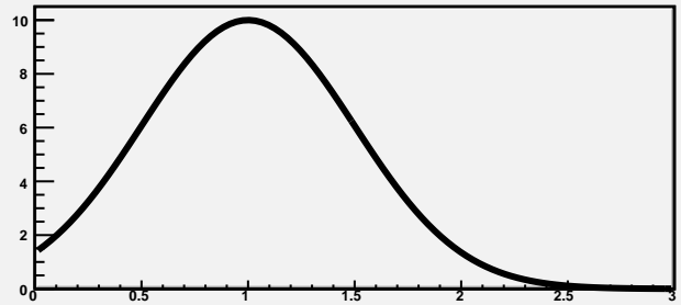
Histogram from a gaussian
