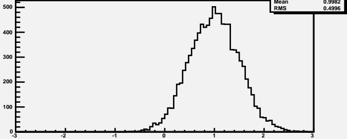
Histogram from my function
