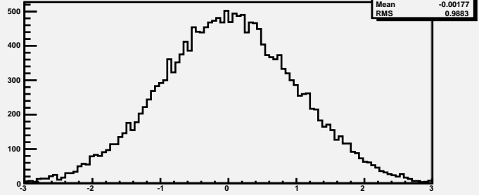
Histogram from a gaussian
