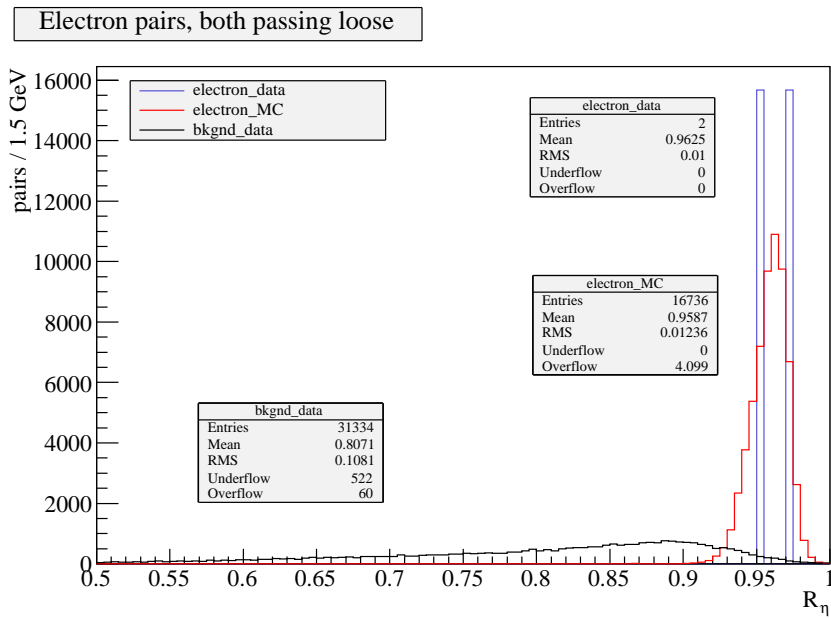
Figure 1: This Histogram shows R_\eta values for real data, simulated data as well as background
