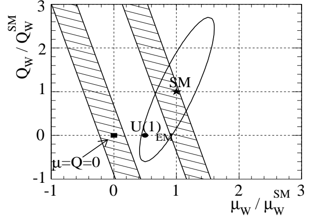
FIG. 14. The W boson electric quadrupole moment vs magnetic dipole moment from W\gamma production relative to their SM values. The ellipse shows the 95% confidence level limit from the D0 experiment with both Q and \mu allowed to vary. Limits from b \rightarrow s\gamma from CLEO at Cornell and ALEPH at LEP are shown as the hatched bands. The star shows the moments if the SM couplings are correct; the filled circle corresponds to a SM SU(2) coupling of zero.
