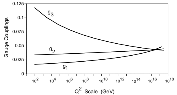
FIG. 16. Gauge couplings g_1, g_2, g_3 as a function of q^2 in the context of the minimal supersymmetric model, showing unification around 10^{16} GeV.
