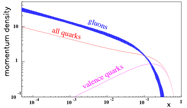
FIG. 2. The quark and gluon momentum densities in the proton versus x for Q^2 = 20 \text{ GeV}^2 . The integrated values of each component density gives the fraction of the proton momentum carried by that component. The valence u and d quarks carry the quantum numbers of the proton. The large number of quarks at small x arise from a 'sea' of quark-antiquark pairs. The quark densities are from a phenomenological fit (CTEQ) to data from many sources; the gluon density bands are the one standard deviation bounds to QCD fits to ZEUS data (low x ) and muon scattering data (higher x ).
