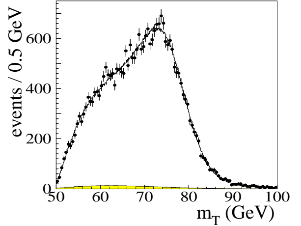
FIG. 10. Transverse mass distribution for W \rightarrow e\nu from the DØ experiment. The transverse mass is defined as M_T = (2E_T^e E_T^\nu (1 - \cos \phi^{e\nu}))^{1/2} with E_T^e and E_T^\nu the transverse energies of electron and neutrino and \phi^{e\nu} the azimuthal angle between them. M_T has its Jacobian edge at the mass of the W boson.
