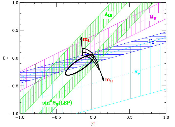
FIG. 12. Several precise electroweak measurements are presented in terms of the S and T variables which characterize the consistency of many experimental observables and the SM. The bands shown from the experimental measurements of A_{LR} (SLC), \Gamma_Z (LEP), \sin^2 \theta_w (LEP), M_W (FNAL and CERN) and R_\nu ( \nu deep inelastic scattering experiments at CERN and FNAL) indicate the allowed regions in S, T space. The half-chevron region centered on S = T = 0 gives the prediction for top mass = 175.5 \pm 5.5 GeV and Higgs mass between 70 and 1000 GeV, providing the SM is correct. A fit to all electroweak data yields the 68% confidence region bounded by the ellipse and shows the consistency of the data and the agreement with the minimal SM theory.
