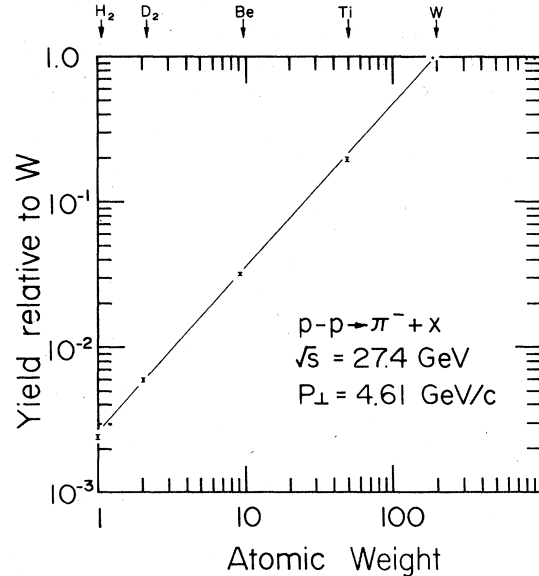
FIG. 12. A plot of the ratio of the cross section for the production of \pi^- per nucleus for H_2 , D_2 , Be, Ti, and W targets, normalized to the W yield, plotted versus the atomic weight. The solid line is the power-law fit of the form A^{\alpha(p_{\perp})} . The fit is only to the four complex nucleus data points.
