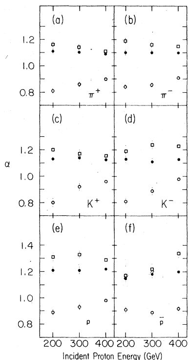
FIG. 19. The energy dependence of the power \alpha of the A dependence of the invariant cross section for the production of hadrons by protons. The points with open circles are for p_L = 0.77 GeV/c, with closed circles for p_L = 3.08 GeV/c, and open squares for p_L = 4.62 GeV/c; (a) \pi^+ , (b) \pi^- , (c) K^+ , (d) K^- , (e) p , (f) \bar{p} . Unless indicated, the errors are smaller than or equal to the size of the points.
