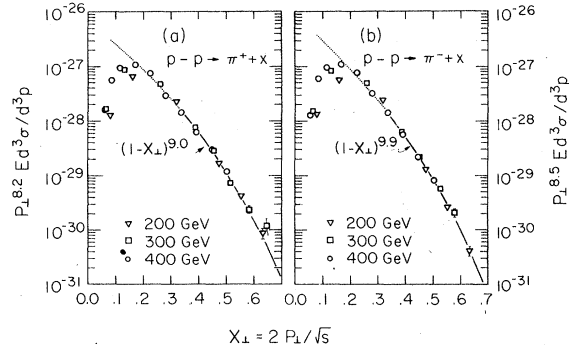
FIG. 3. The scaling properties of the \pi^+ and \pi^- cross sections versus x_1 = 2p_\perp/\sqrt{s} . The cross sections have been multiplied by p_\perp^n , where n is the best-fit value. The solid line is the fitted parametrization. The fit is over the region x_1 > 0.35 .
