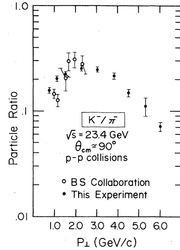
FIG. 8. A comparison of the K^-/\pi^- ratio versus p_{\perp} with the BS collaboration (Ref. 15) at \sqrt{s} = 23.4 GeV/ c^2 .
