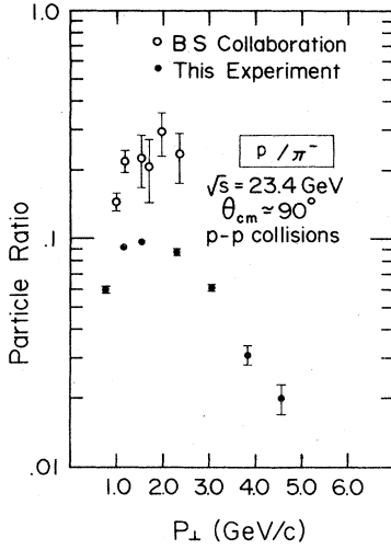
FIG. 10. A comparison of the \bar{p}/\pi^- ratio versus p_\perp with the BS collaboration (Ref. 15) at \sqrt{s} = 23.4 GeV/ c^2 .
