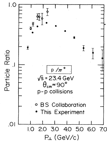
FIG. 9. A comparison of the p/\pi^+ ratio versus p_{\perp} with the BS collaboration (Ref. 15) at \sqrt{s} = 23.4 GeV/ c^2 .
