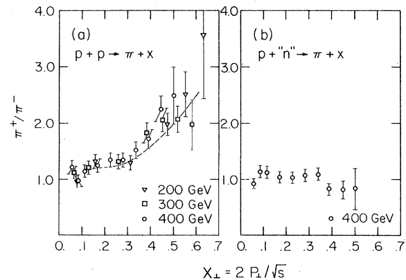
FIG. 5. The ratio of \pi^+ to \pi^- production versus x_1 for 200-, 300-, and 400-GeV incident protons. The left-hand plot is for p - p collisions; the right-hand for p -" n " collisions. The dashed line is the Feynman-Field-Fox QCD prediction of Ref. 12 for \sqrt{s} = 19.4 GeV/ c^2 .
