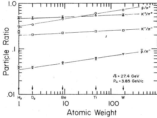
FIG. 15. A plot of the particle ratios versus atomic weight A at a p_L of 3.85 GeV/c. The lines are fits of the form A^{\Delta\alpha(\phi_L)} .
