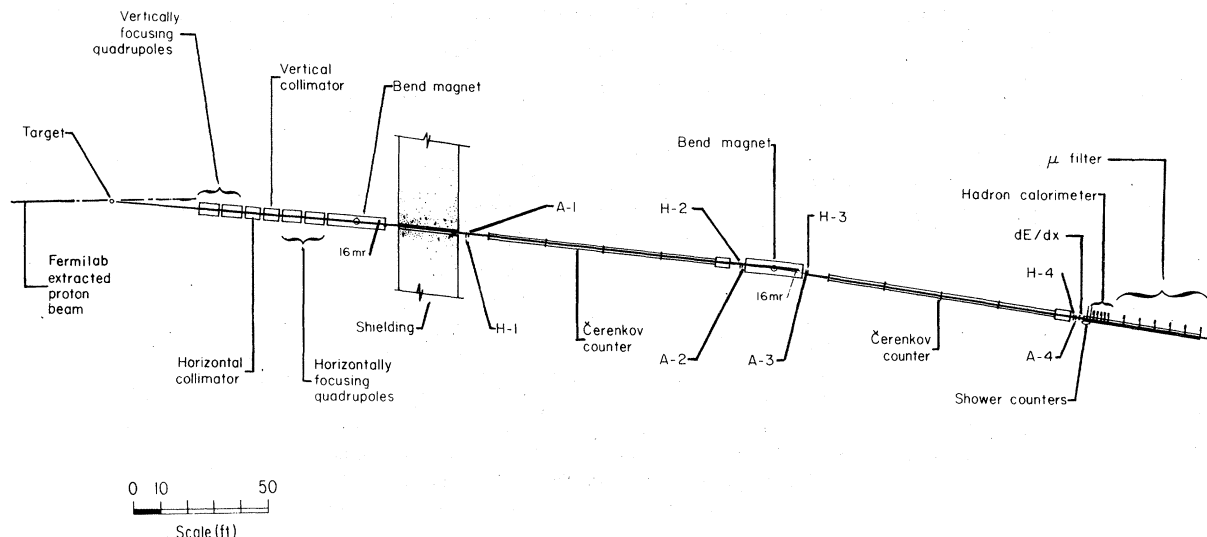
FIG. 1. The spectrometer.
