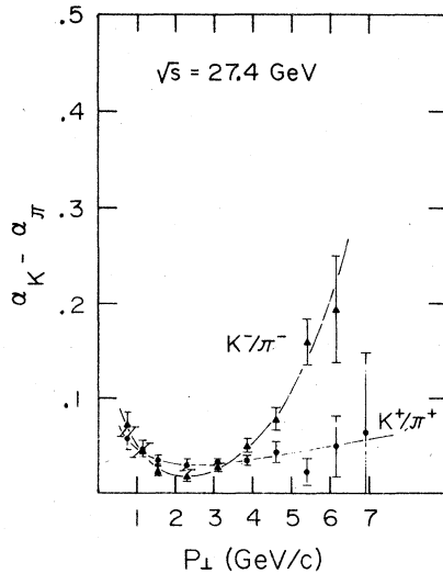
FIG. 16. The value of the differences \alpha_K - \alpha_\pi derived from the particle ratios versus p_L at 400 GeV/c. The lines are drawn to guide the eye.
